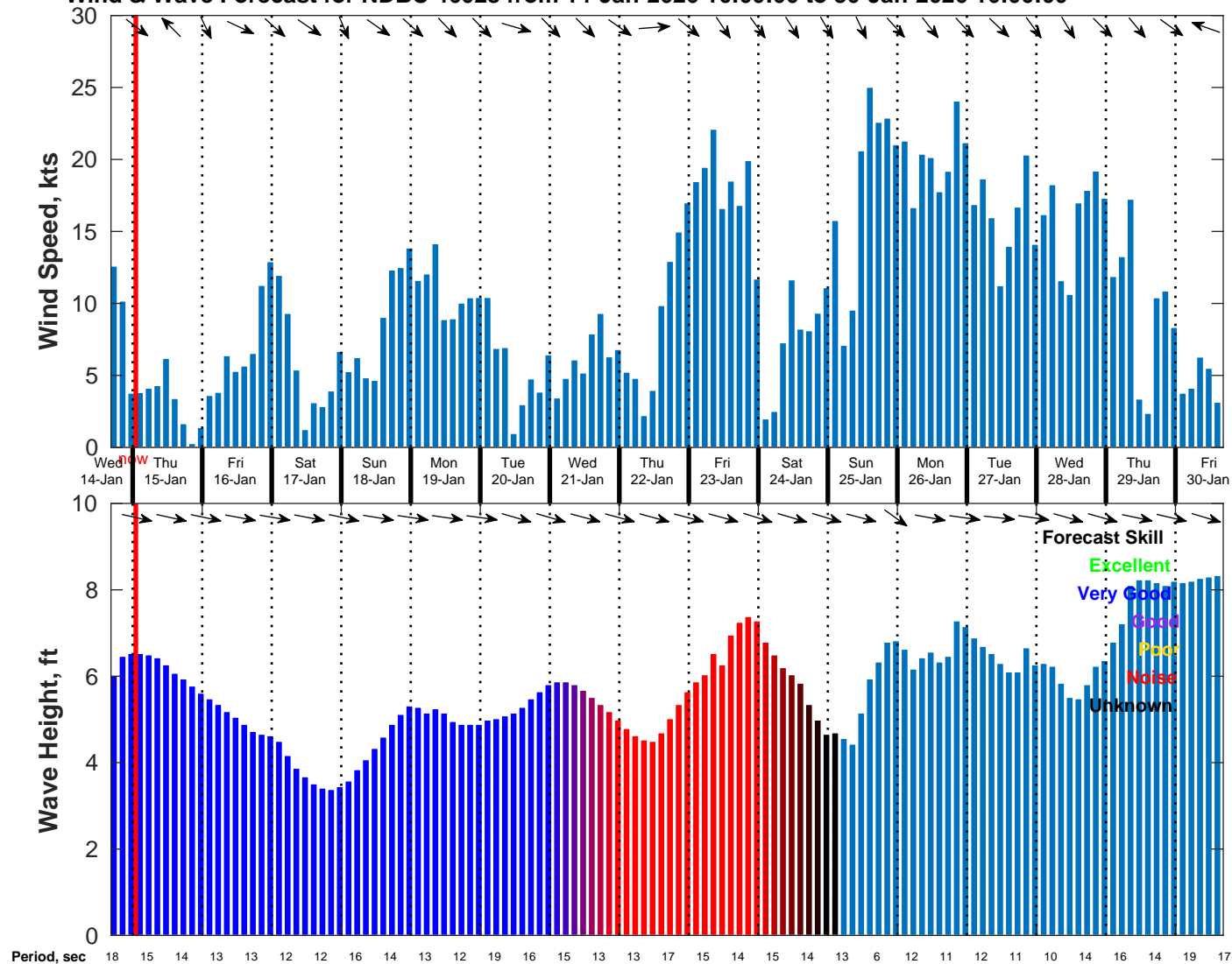
Wind & Wave Forecast for NDBC 46028 from 14-Jan-2026 16:00:00 to 30-Jan-2026 16:00:00
