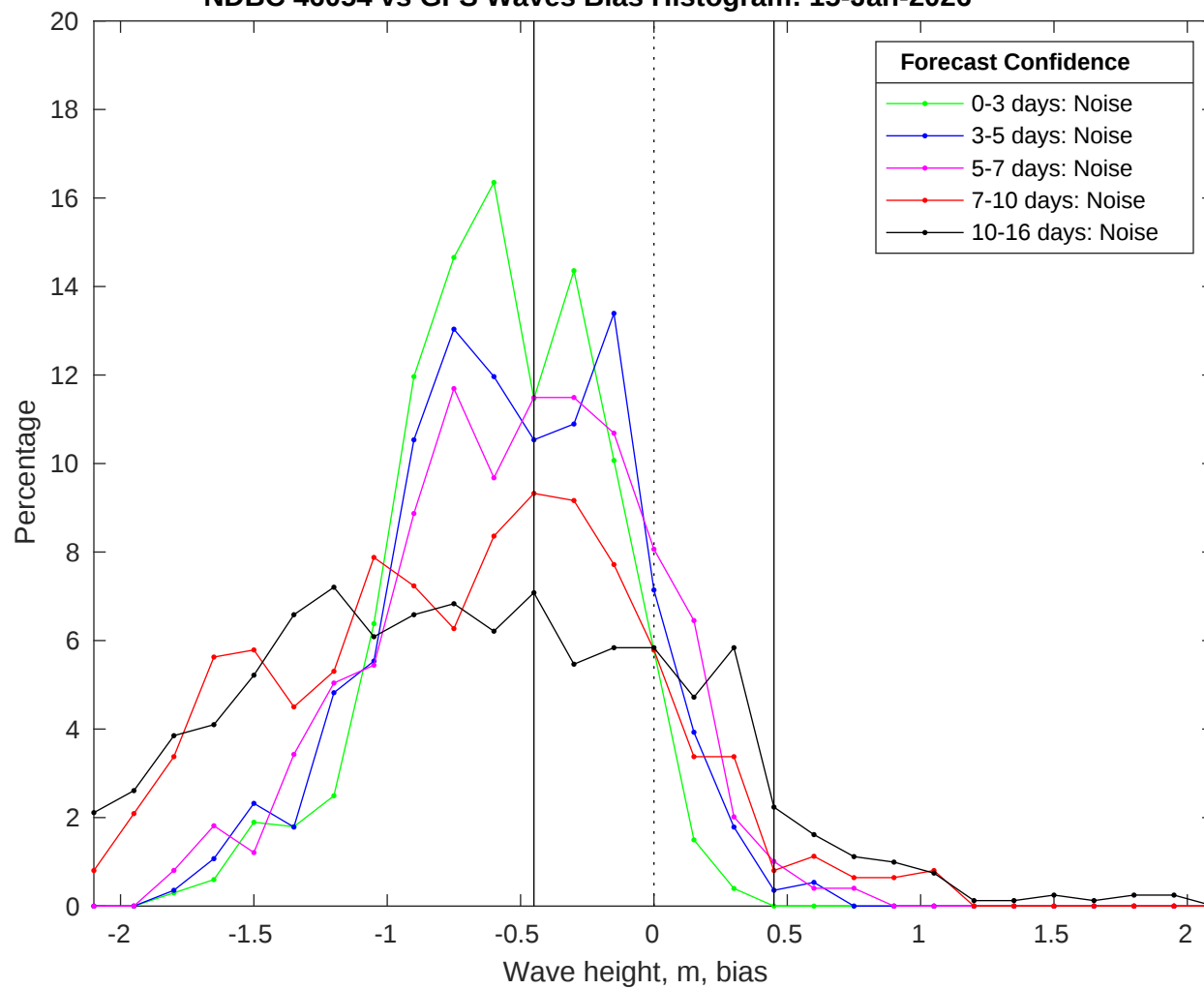
NDBC 46054 vs GFS Waves Bias Histogram: 15-Jan-2026
