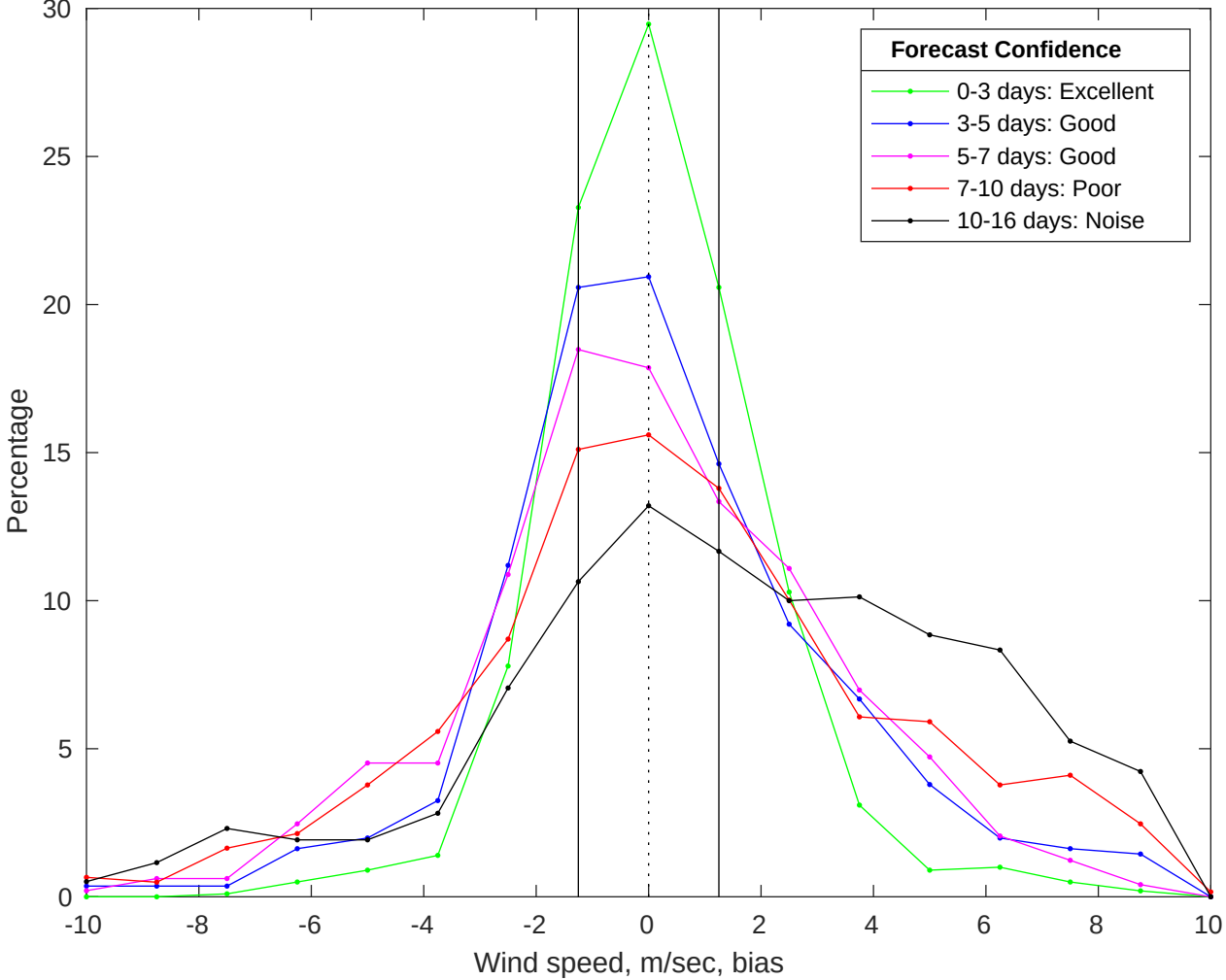
NDBC 46054 vs GFS Winds Bias Histogram: 15-Jan-2026
