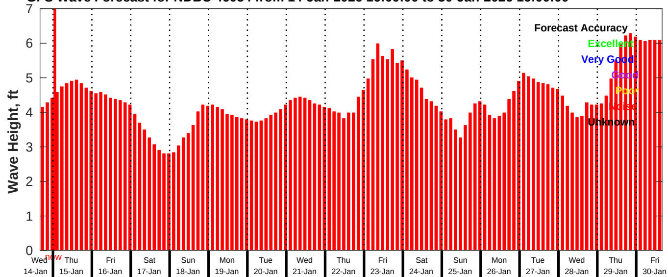
GFS Wave Forecast for NDBC 46054 from 14-Jan-2026 16:00:00 to 30-Jan-2026 16:00:00
