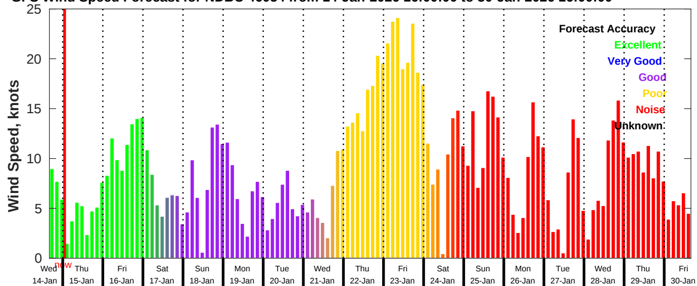
GFS Wind Speed Forecast for NDBC 46054 from 14-Jan-2026 16:00:00 to 30-Jan-2026 16:00:00
