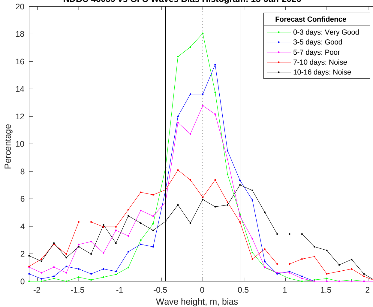
NDBC 46059 vs GFS Waves Bias Histogram: 15-Jan-2026
