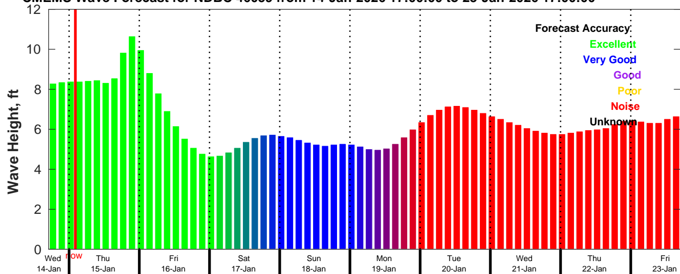
CMEMS Wave Forecast for NDBC 46059 from 14-Jan-2026 17:00:00 to 23-Jan-2026 17:00:00
