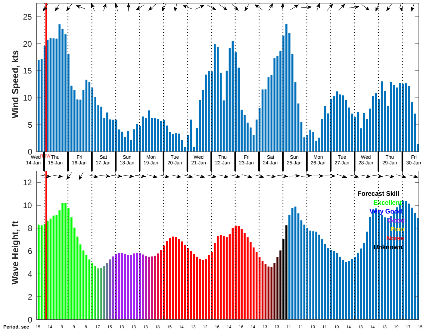
Wind & Wave Forecast for NDBC 46059 from 14-Jan-2026 17:00:00 to 30-Jan-2026 17:00:00
