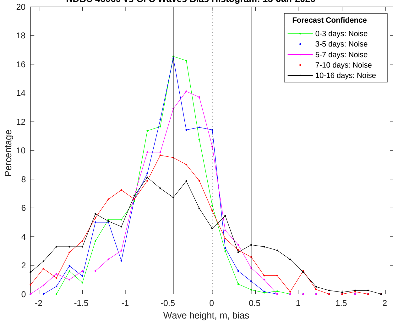
NDBC 46069 vs GFS Waves Bias Histogram: 15-Jan-2026
