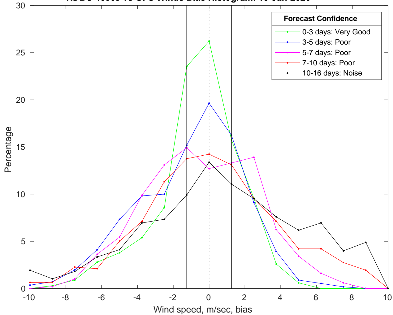
NDBC 46069 vs GFS Winds Bias Histogram: 15-Jan-2026
