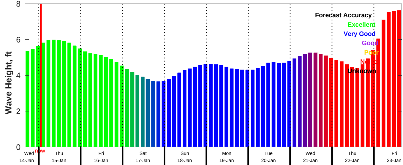
CMEMS Wave Forecast for NDBC 46069 from 14-Jan-2026 16:00:00 to 23-Jan-2026 16:00:00
