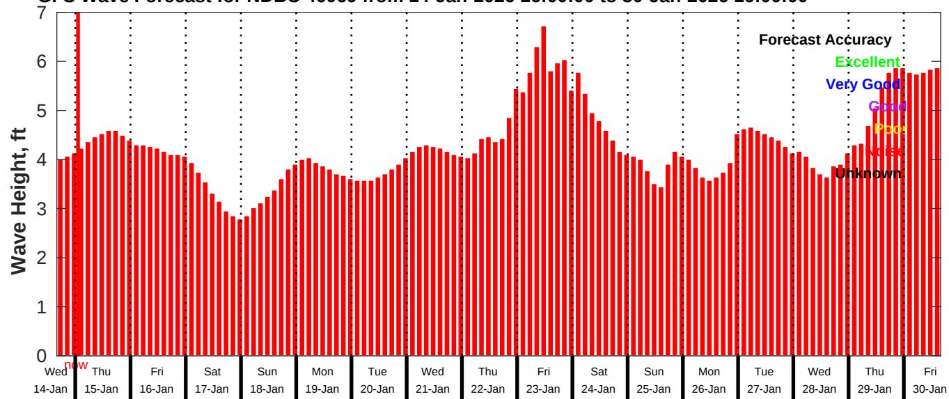
GFS Wave Forecast for NDBC 46069 from 14-Jan-2026 16:00:00 to 30-Jan-2026 16:00:00
