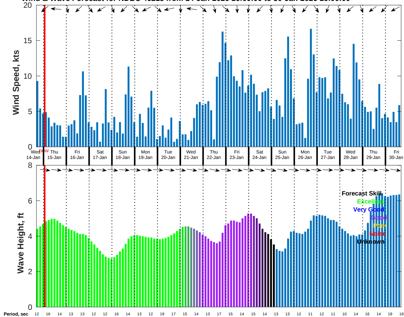
Wind & Wave Forecast for NDBC 46215 from 14-Jan-2026 16:00:00 to 30-Jan-2026 16:00:00
