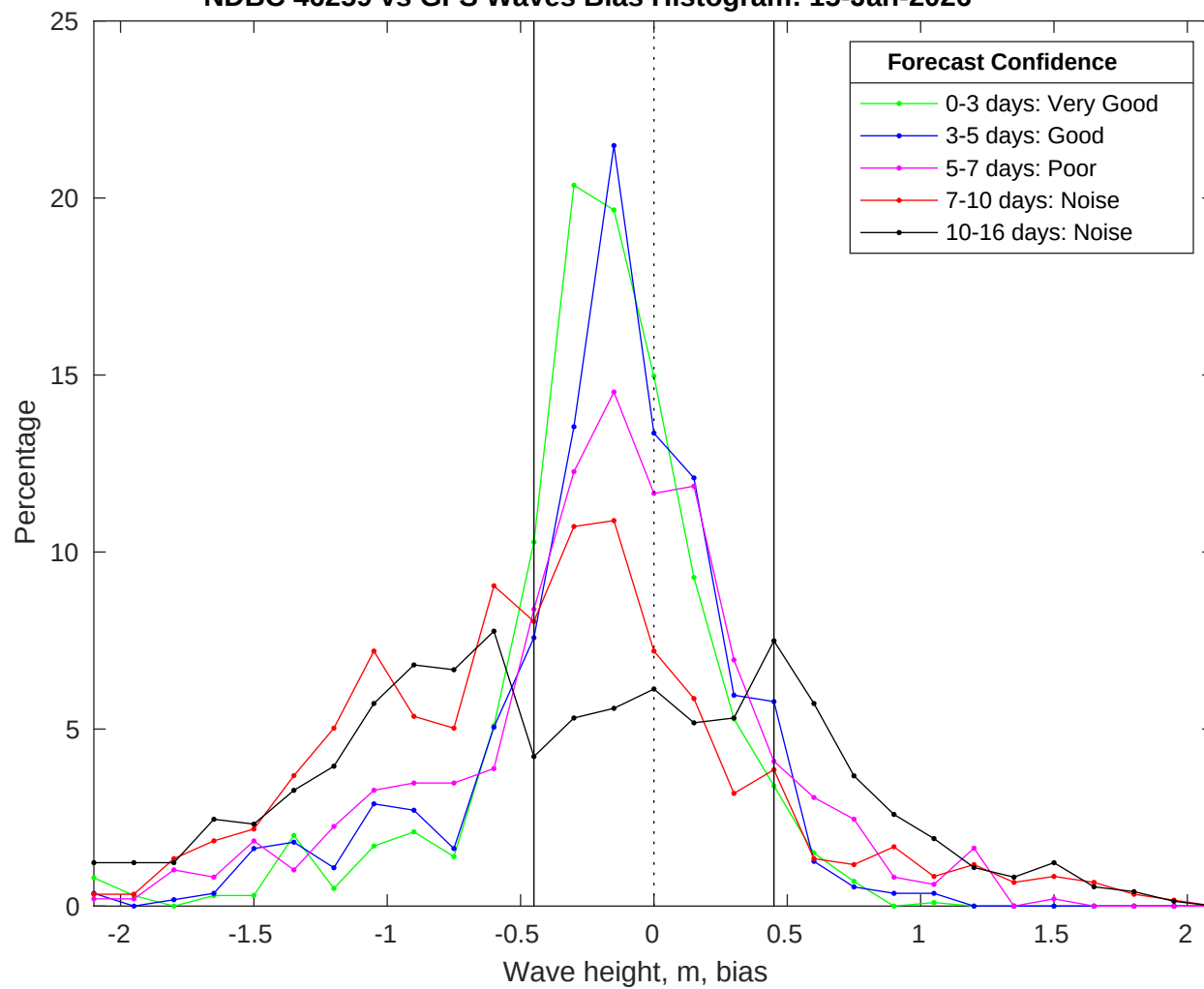
NDBC 46259 vs GFS Waves Bias Histogram: 15-Jan-2026
