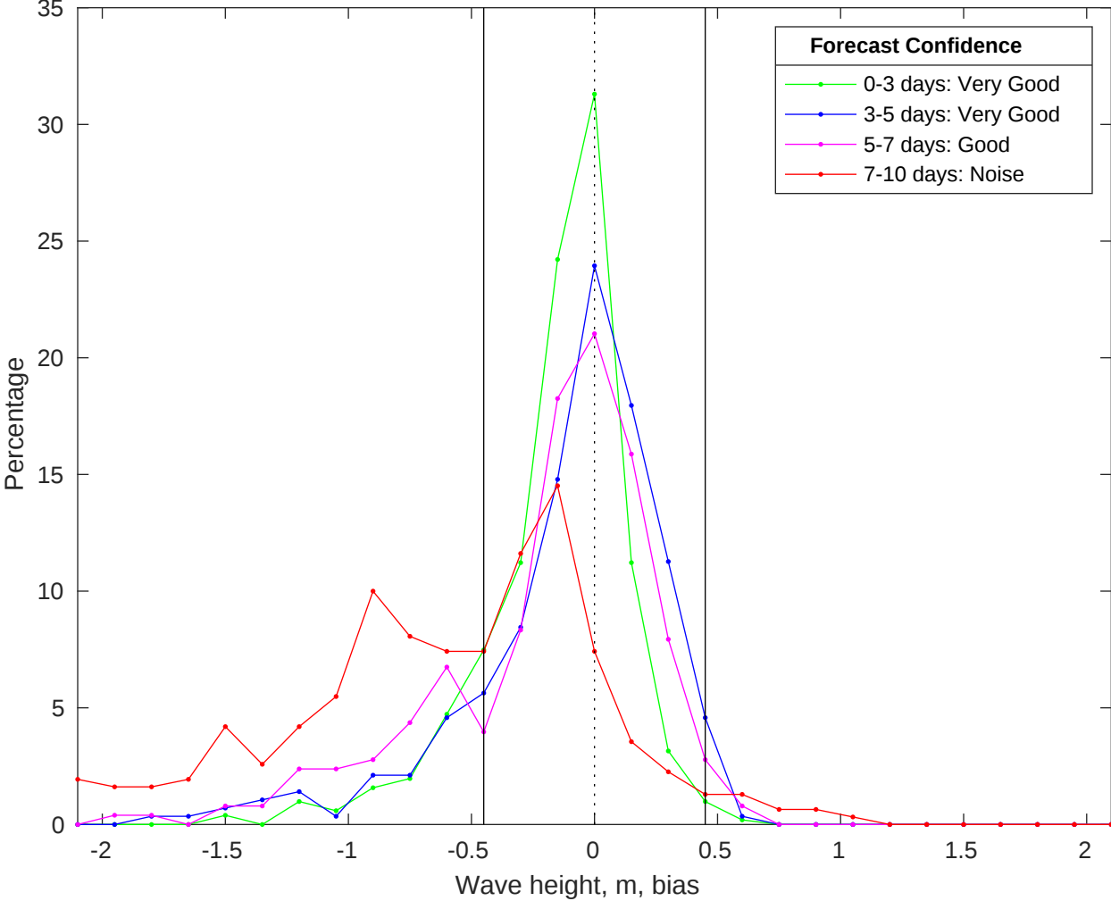
NDBC 51000 vs CMEMS Waves Bias Histogram: 15-Jan-2026
