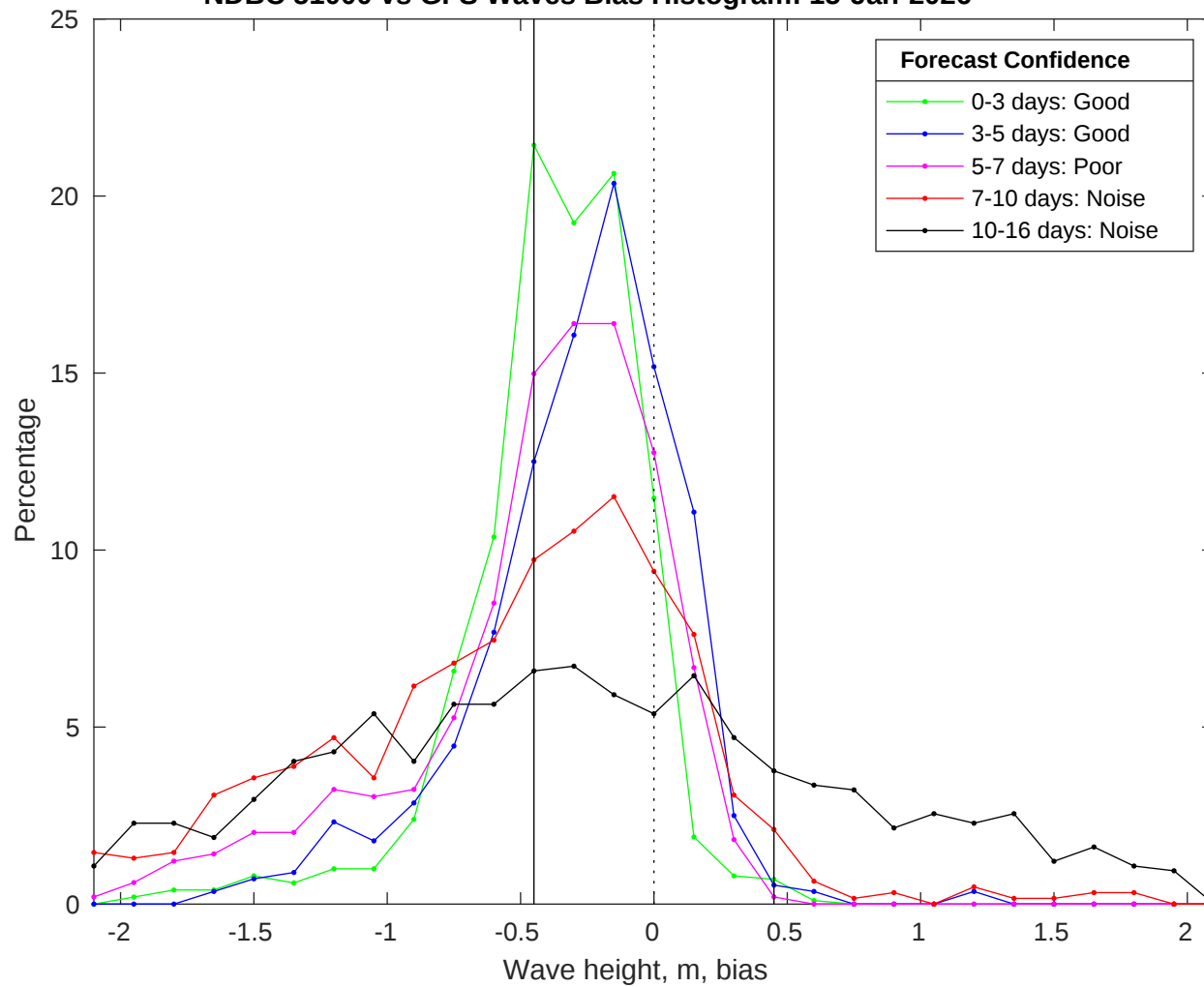
NDBC 51000 vs GFS Waves Bias Histogram: 15-Jan-2026
