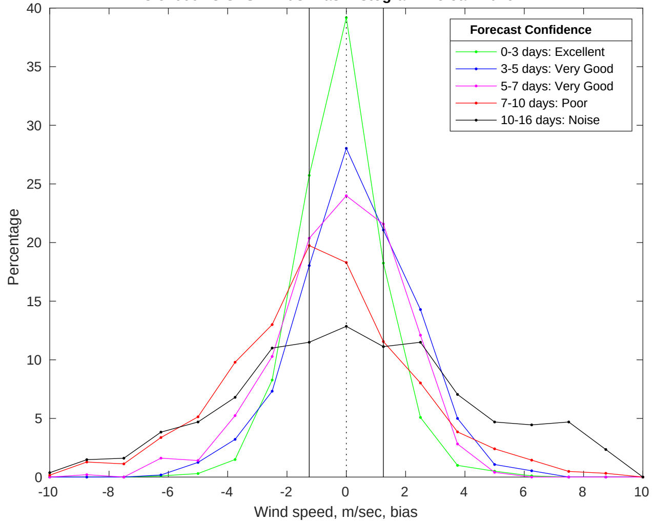
NDBC 51000 vs GFS Winds Bias Histogram: 15-Jan-2026
