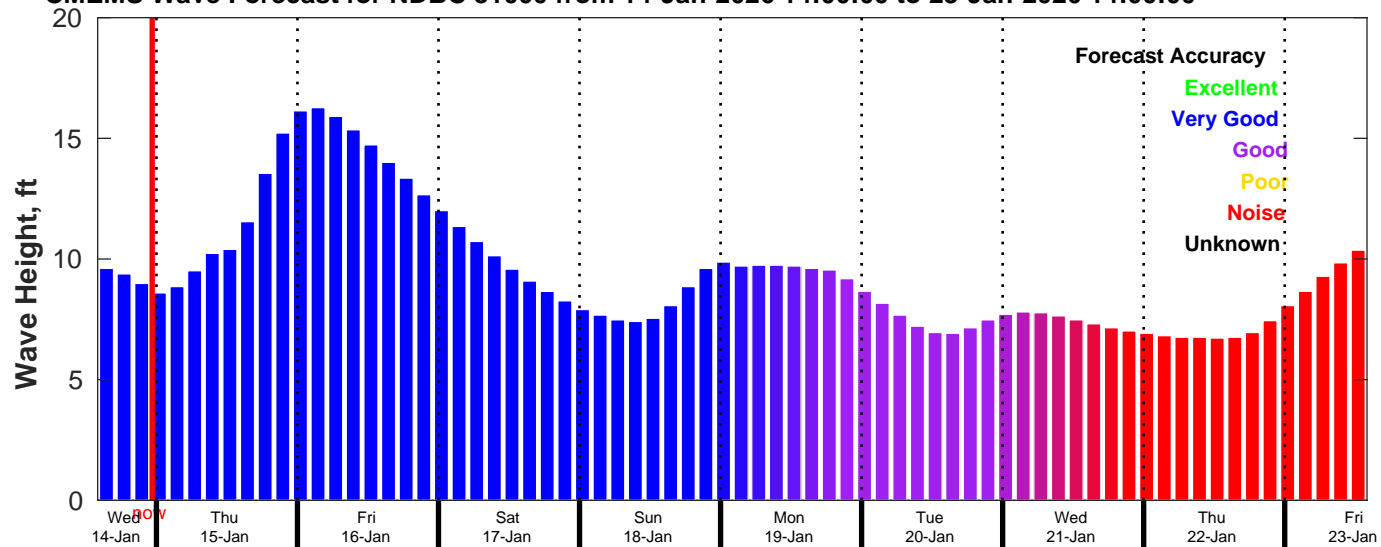
CMEMS Wave Forecast for NDBC 51000 from 14-Jan-2026 14:00:00 to 23-Jan-2026 14:00:00
