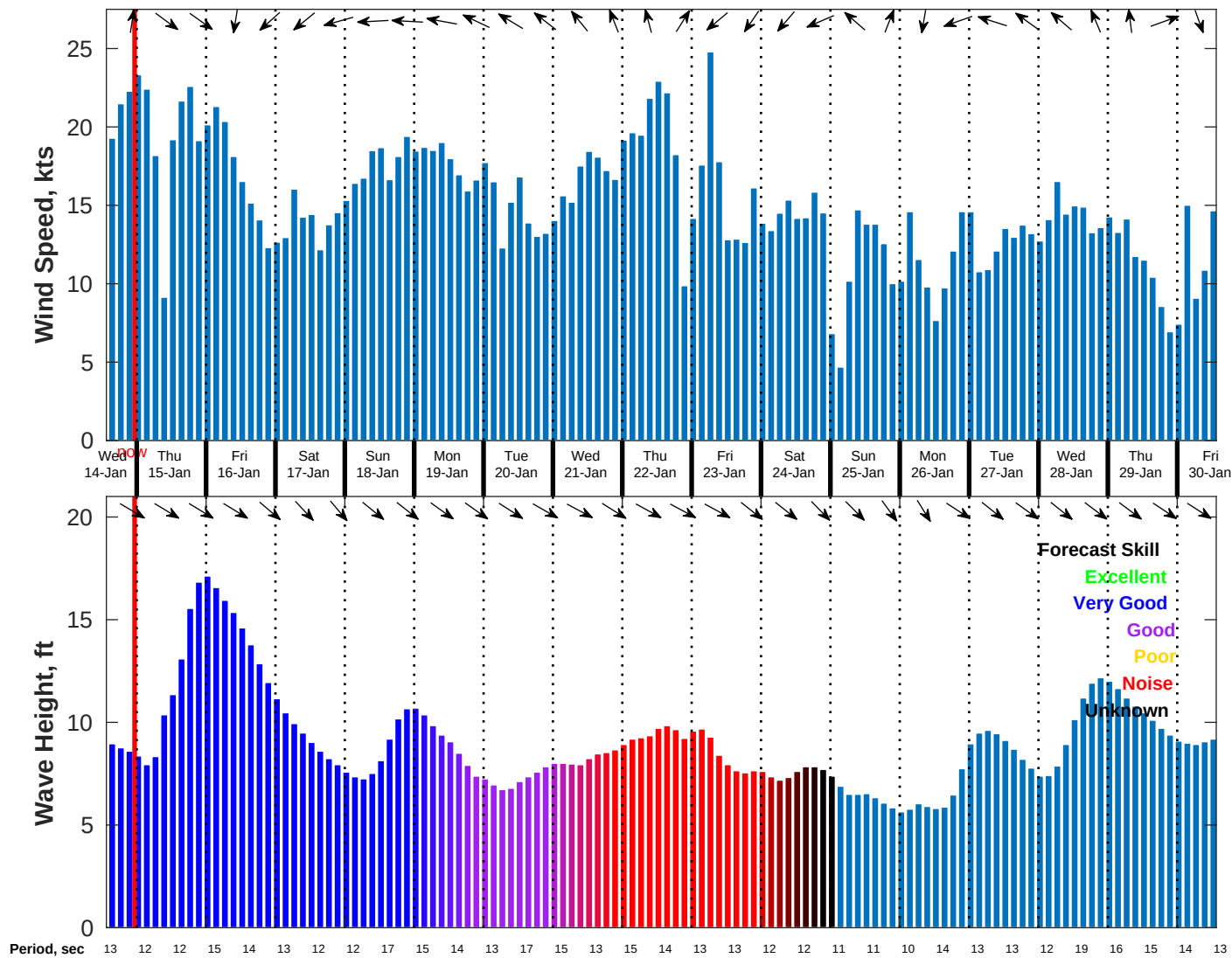
Wind & Wave Forecast for NDBC 51000 from 14-Jan-2026 14:00:00 to 30-Jan-2026 14:00:00
