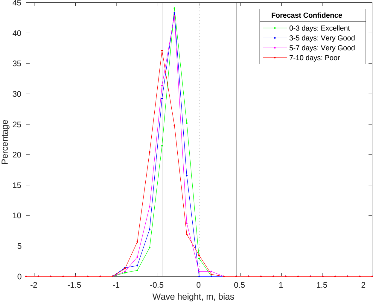
NDBC 51209 vs CMEMS Waves Bias Histogram: 15-Jan-2026
