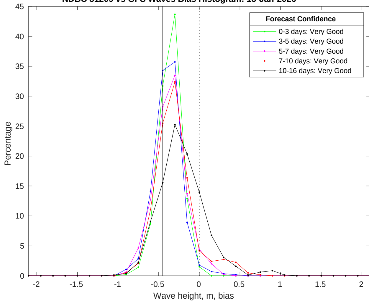
NDBC 51209 vs GFS Waves Bias Histogram: 15-Jan-2026
