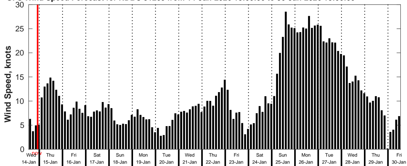
GFS Wind Speed Forecast for NDBC 51209 from 14-Jan-2026 13:00:00 to 30-Jan-2026 13:00:00
