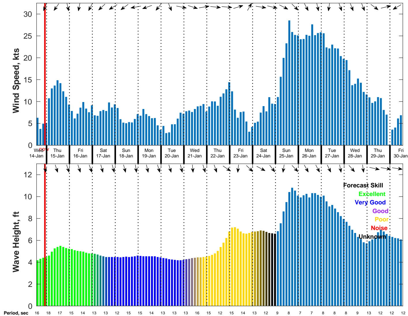
Wind & Wave Forecast for NDBC 51209 from 14-Jan-2026 13:00:00 to 30-Jan-2026 13:00:00
