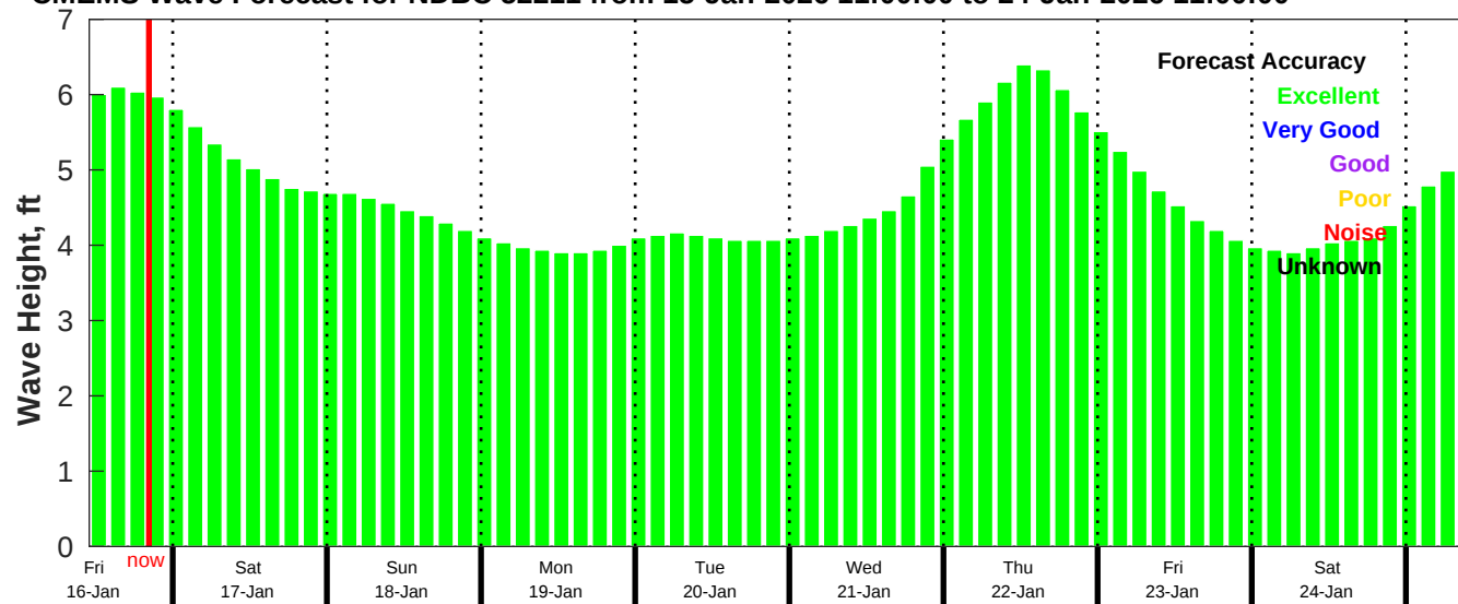
CMEMS Wave Forecast for NDBC 52211 from 15-Jan-2026 11:00:00 to 24-Jan-2026 11:00:00
