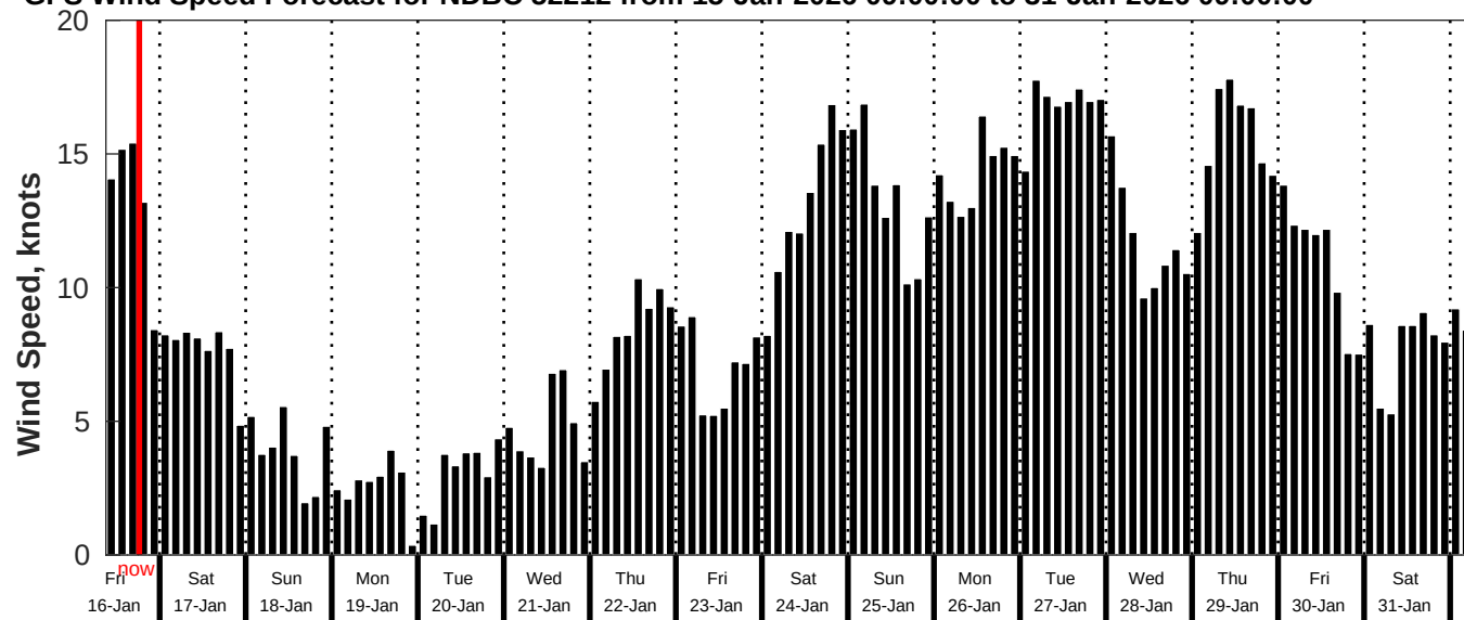
GFS Wind Speed Forecast for NDBC 52212 from 15-Jan-2026 09:00:00 to 31-Jan-2026 09:00:00
