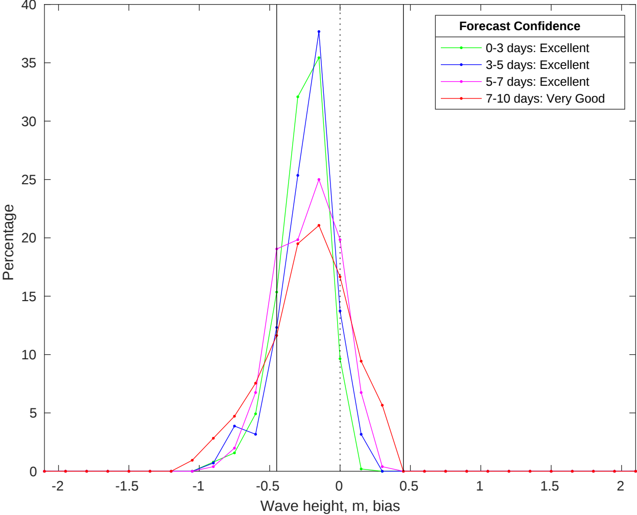
NDBC 52213 vs CMEMS Waves Bias Histogram: 15-Jan-2026
