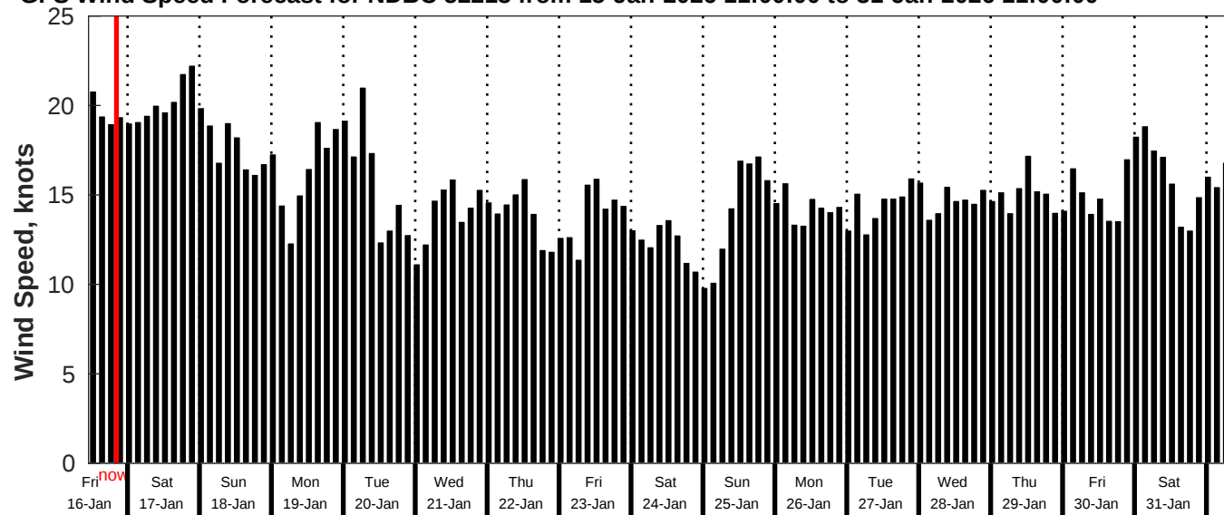
GFS Wind Speed Forecast for NDBC 52213 from 15-Jan-2026 11:00:00 to 31-Jan-2026 11:00:00
