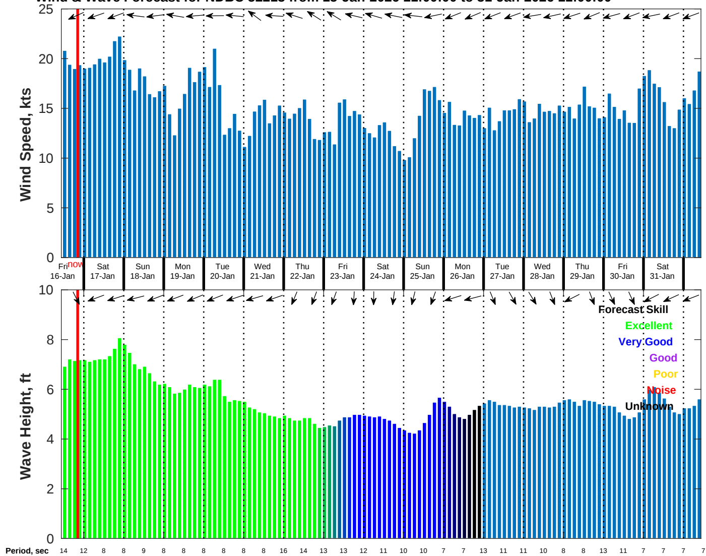
Wind & Wave Forecast for NDBC 52213 from 15-Jan-2026 11:00:00 to 31-Jan-2026 11:00:00
