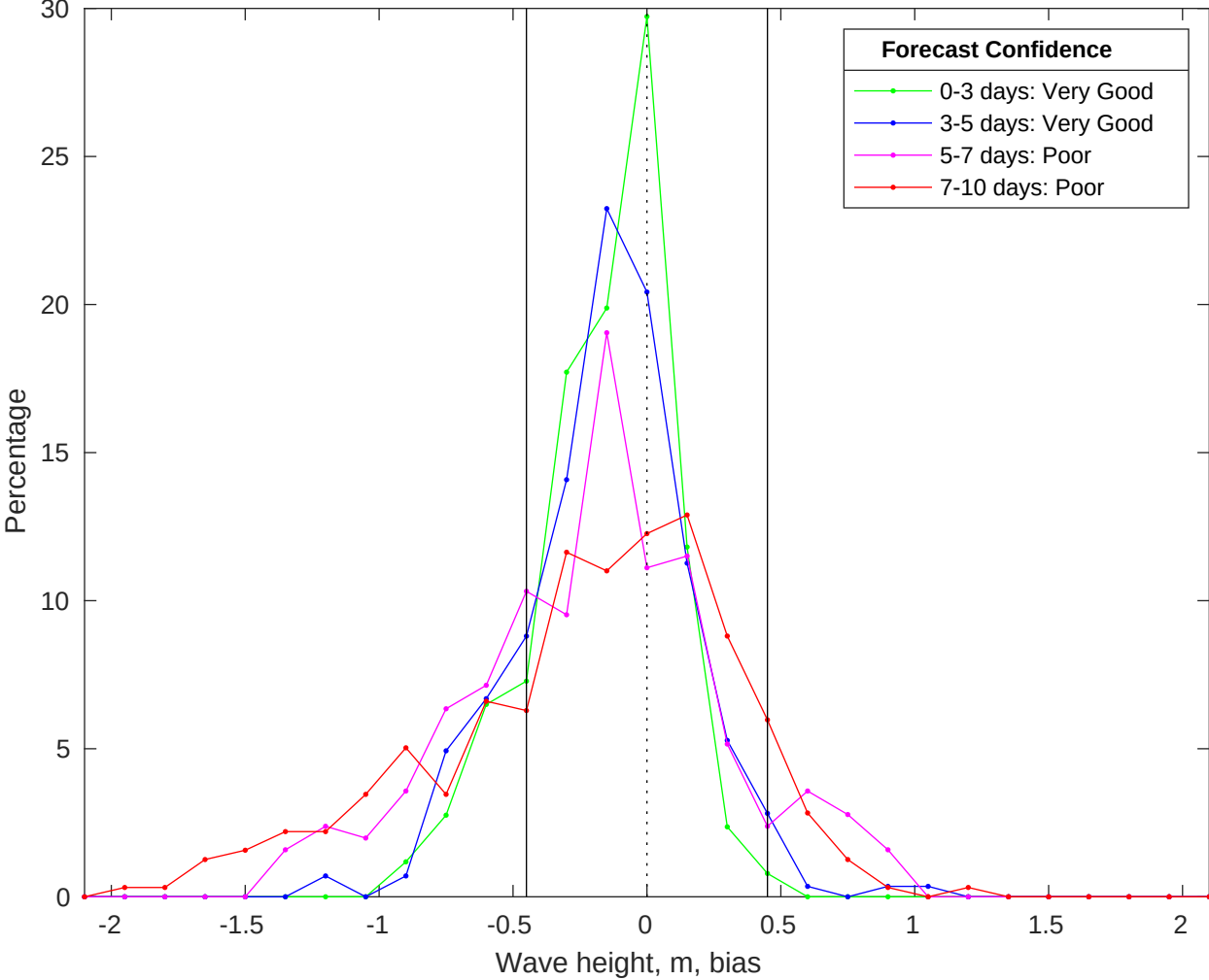
NDBC 41004 vs CMEMS Waves Bias Histogram: 16-Jan-2026
