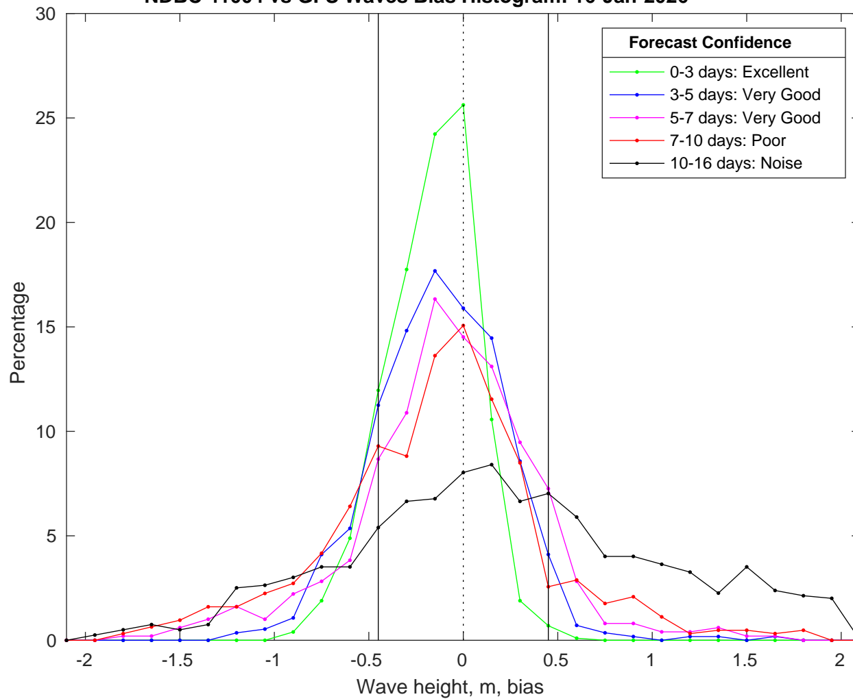
NDBC 41004 vs GFS Waves Bias Histogram: 16-Jan-2026
