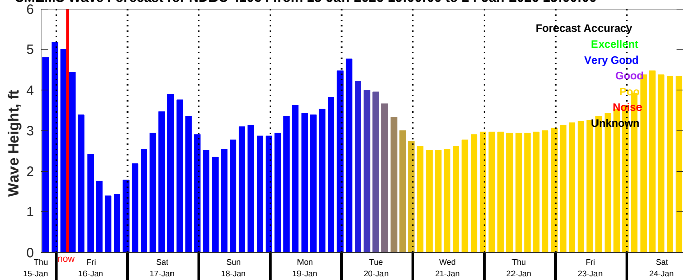
CMEMS Wave Forecast for NDBC 41004 from 15-Jan-2026 19:00:00 to 24-Jan-2026 19:00:00
