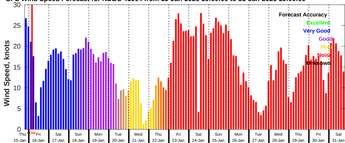
GFS Wind Speed Forecast for NDBC 41004 from 15-Jan-2026 19:00:00 to 31-Jan-2026 19:00:00
