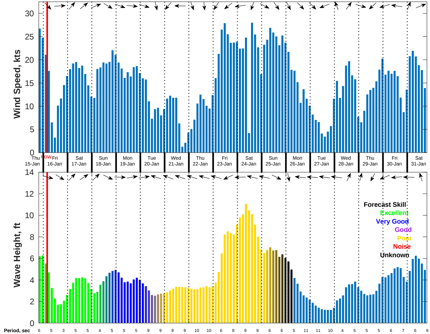
Wind & Wave Forecast for NDBC 41004 from 15-Jan-2026 19:00:00 to 31-Jan-2026 19:00:00
