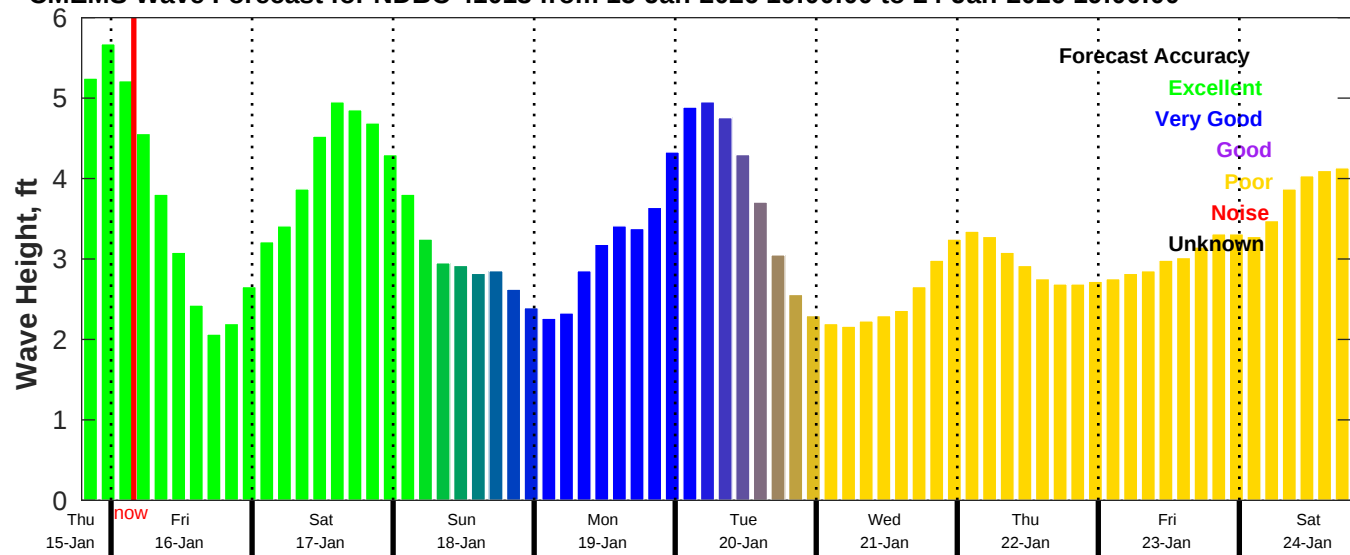
CMEMS Wave Forecast for NDBC 41013 from 15-Jan-2026 19:00:00 to 24-Jan-2026 19:00:00
