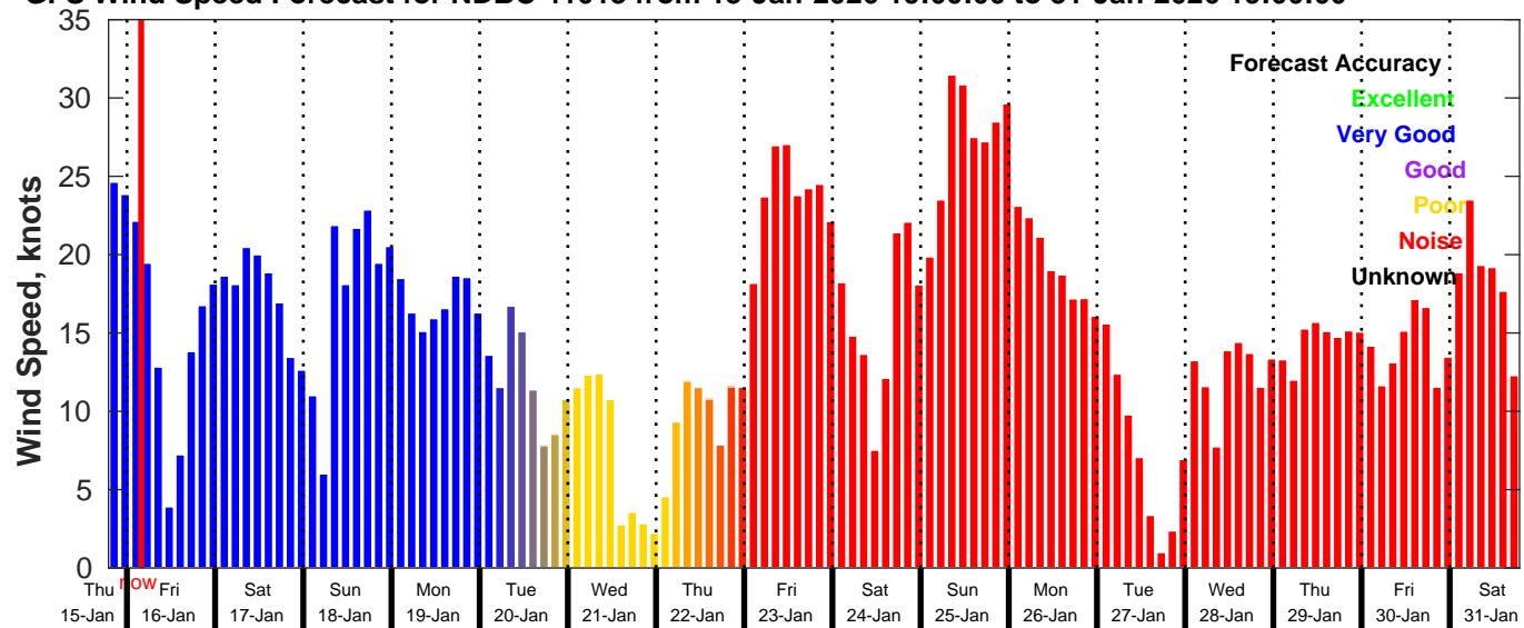
GFS Wind Speed Forecast for NDBC 41013 from 15-Jan-2026 19:00:00 to 31-Jan-2026 19:00:00
