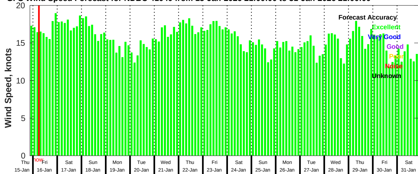
GFS Wind Speed Forecast for NDBC 41040 from 15-Jan-2026 21:00:00 to 31-Jan-2026 21:00:00
