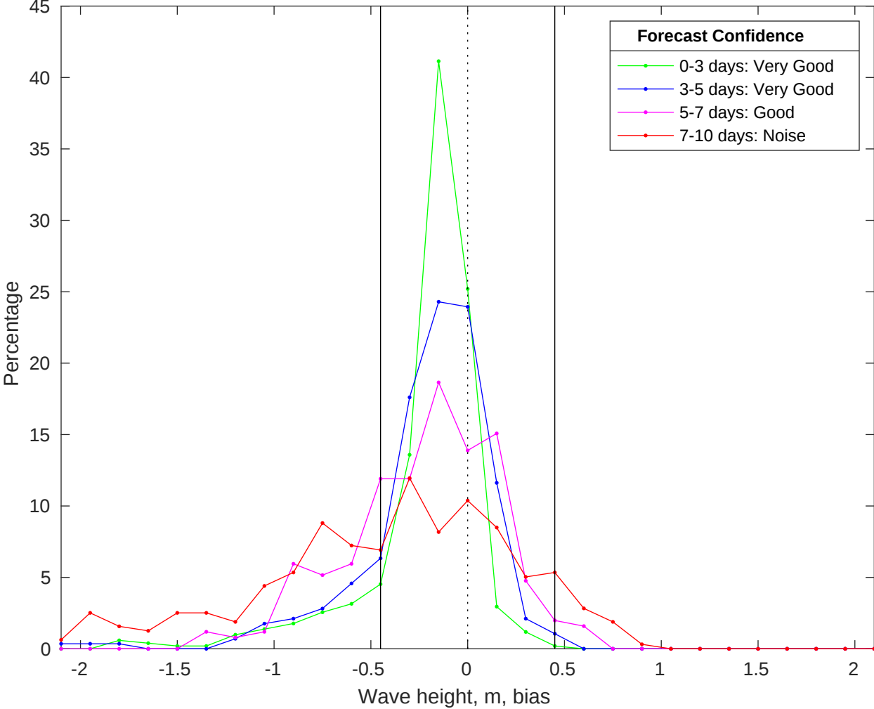
NDBC 42019 vs CMEMS Waves Bias Histogram: 16-Jan-2026
