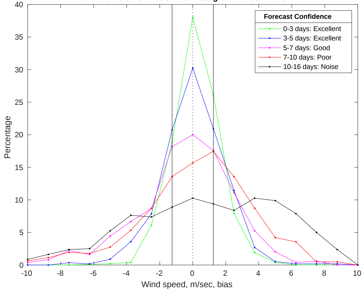
NDBC 42019 vs GFS Winds Bias Histogram: 16-Jan-2026
