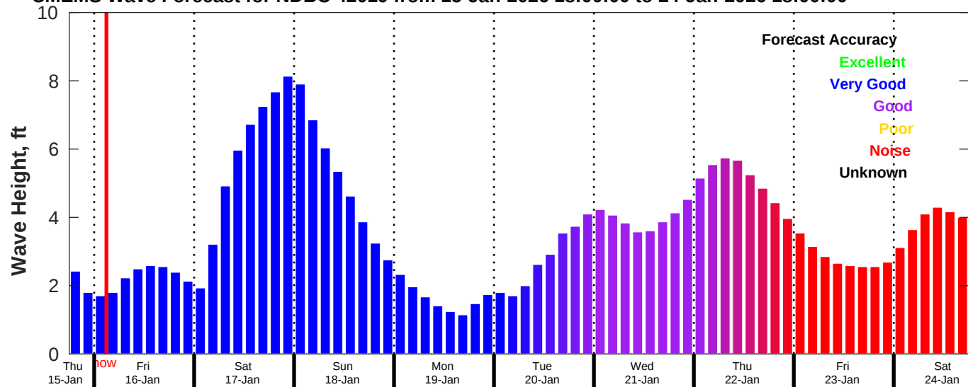
CMEMS Wave Forecast for NDBC 42019 from 15-Jan-2026 18:00:00 to 24-Jan-2026 18:00:00
