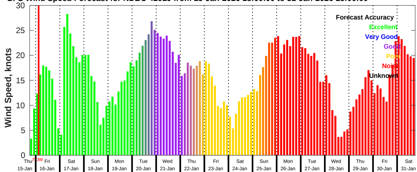
GFS Wind Speed Forecast for NDBC 42019 from 15-Jan-2026 18:00:00 to 31-Jan-2026 18:00:00
