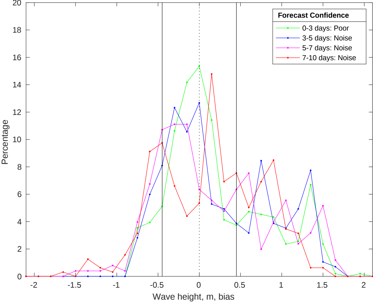
NDBC 42020 vs CMEMS Waves Bias Histogram: 16-Jan-2026
