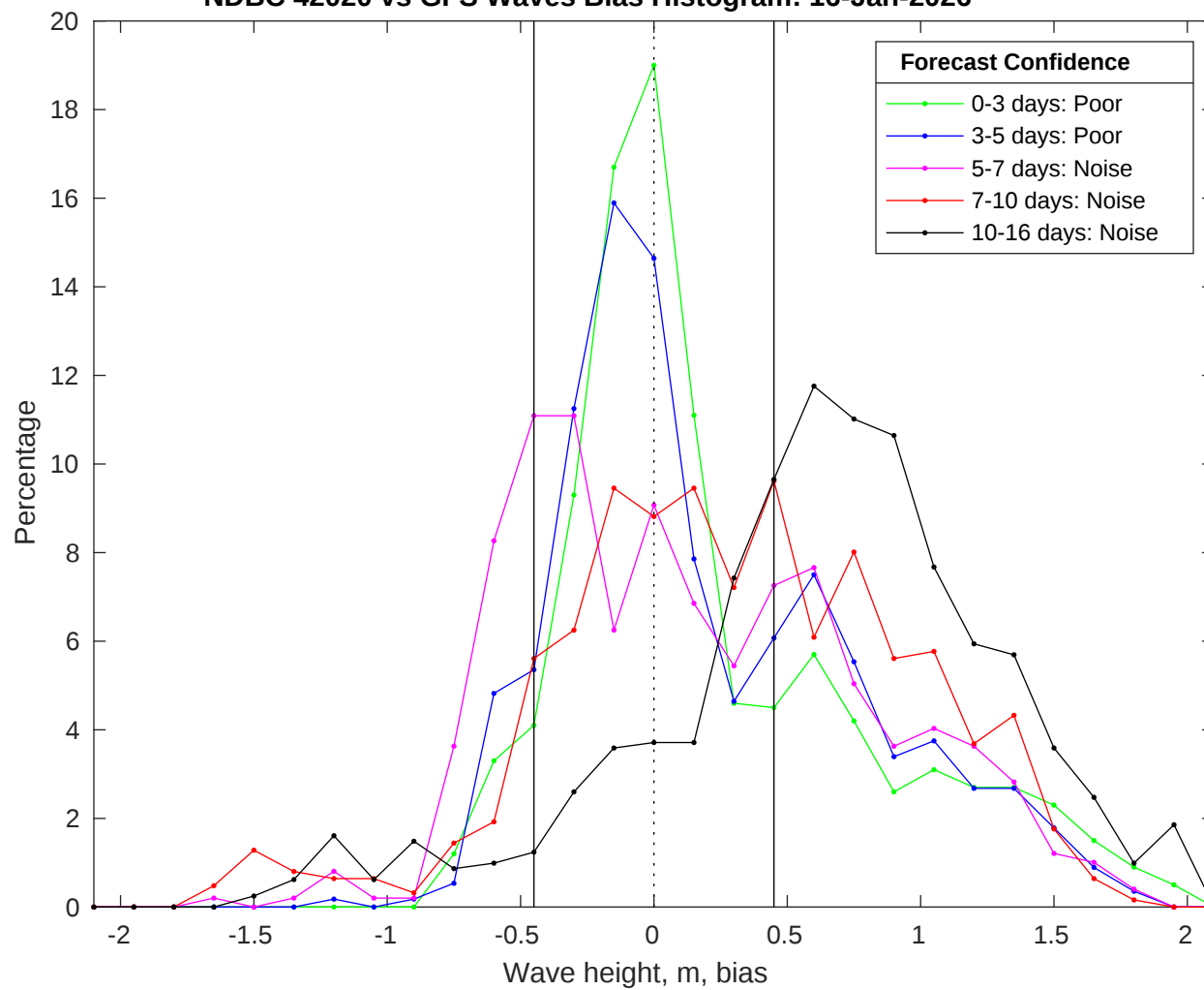
NDBC 42020 vs GFS Waves Bias Histogram: 16-Jan-2026
