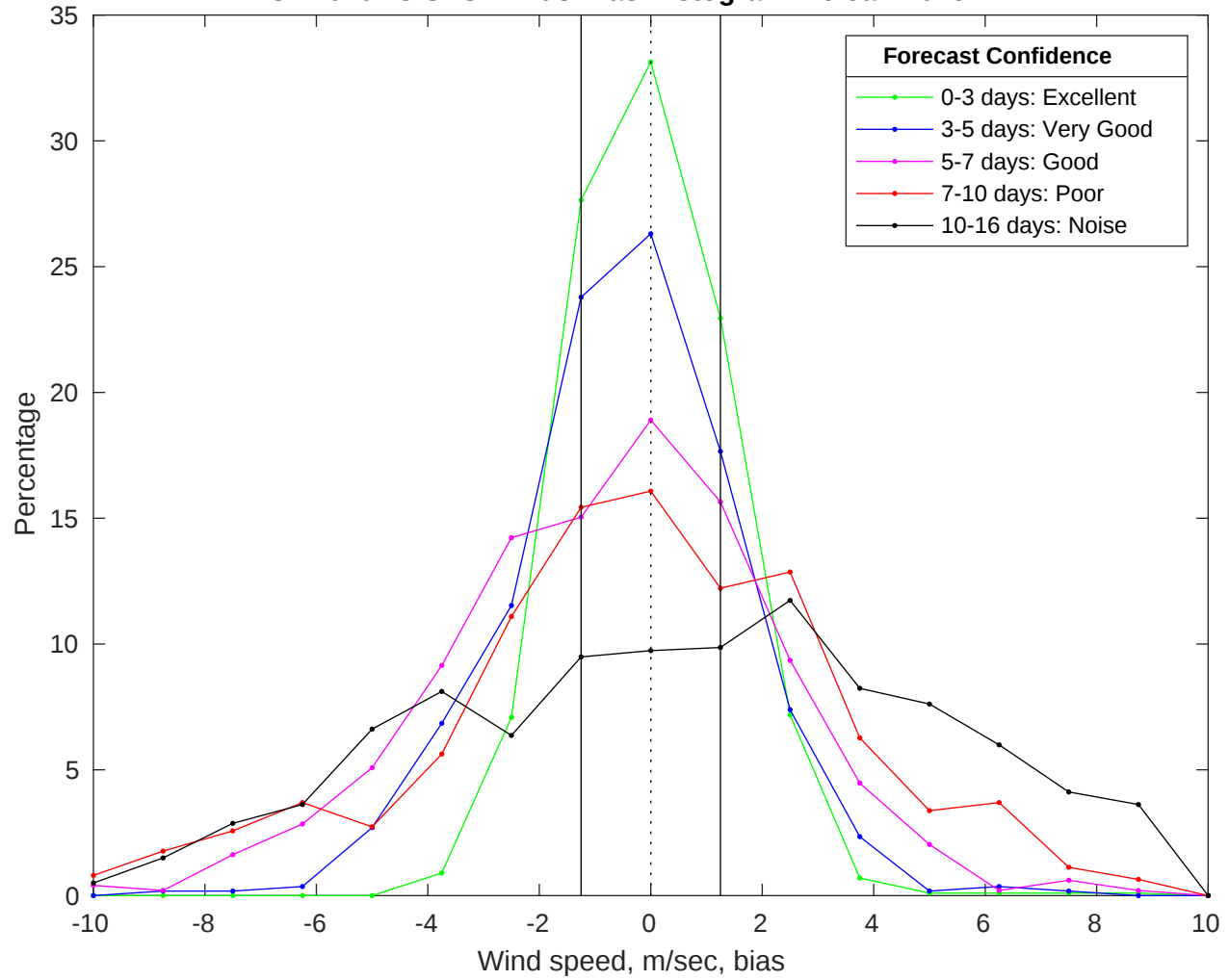
NDBC 42020 vs GFS Winds Bias Histogram: 16-Jan-2026
