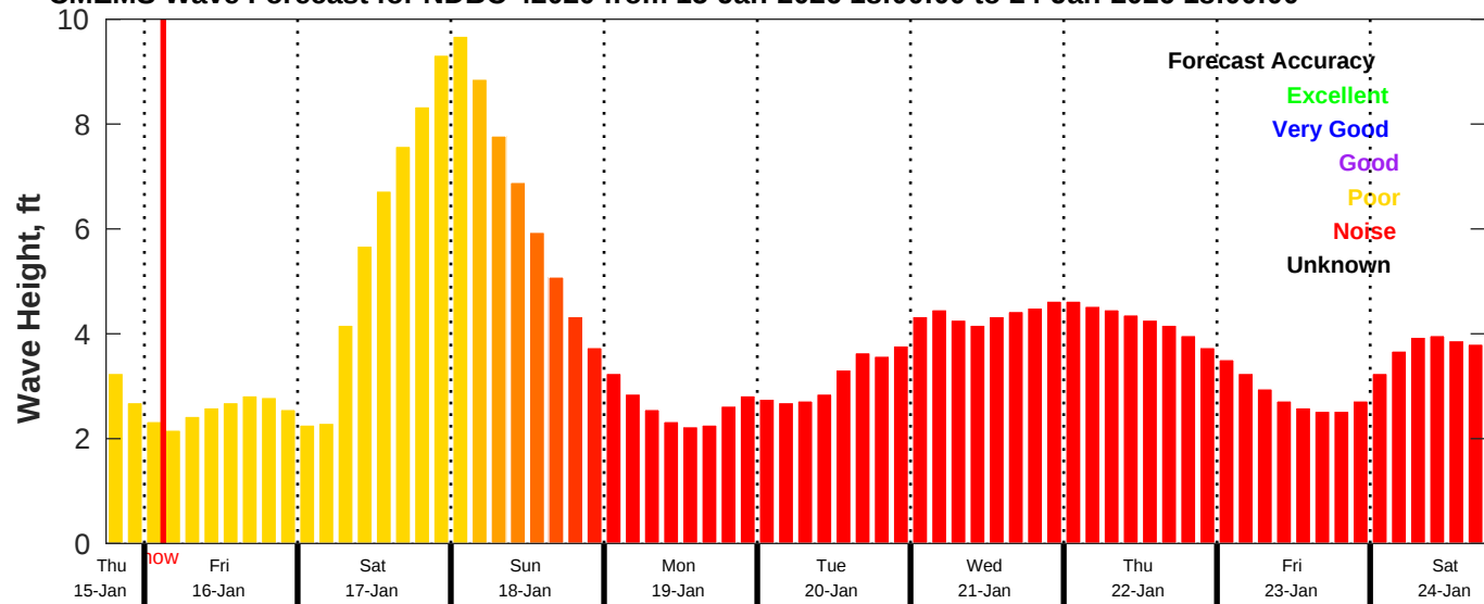
CMEMS Wave Forecast for NDBC 42020 from 15-Jan-2026 18:00:00 to 24-Jan-2026 18:00:00
