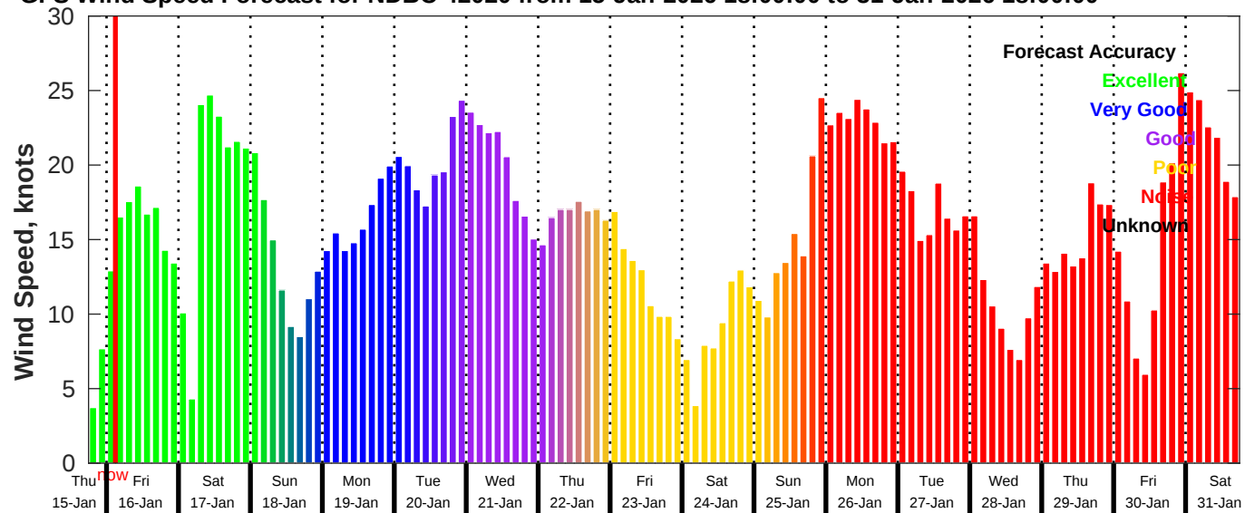
GFS Wind Speed Forecast for NDBC 42020 from 15-Jan-2026 18:00:00 to 31-Jan-2026 18:00:00
