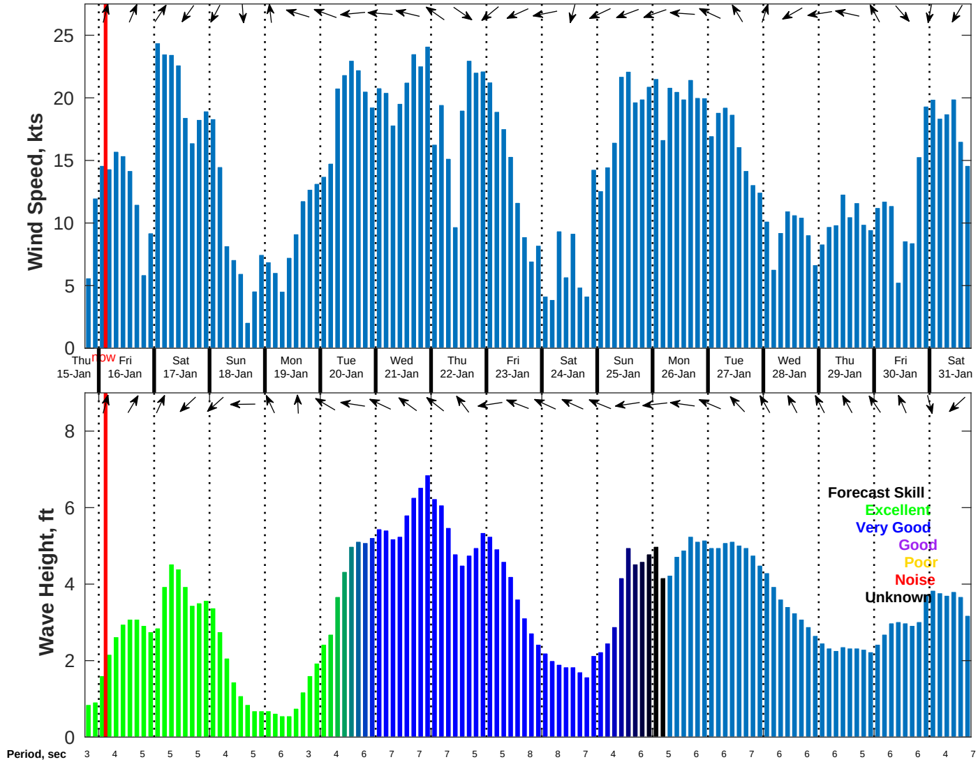
Wind & Wave Forecast for NDBC 42035 from 15-Jan-2026 18:00:00 to 31-Jan-2026 18:00:00
