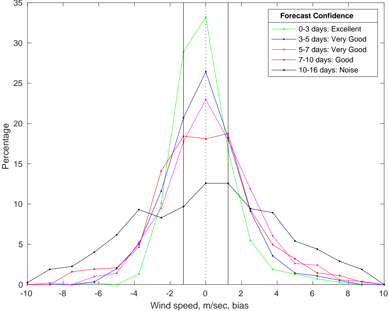
NDBC 42036 vs GFS Winds Bias Histogram: 16-Jan-2026
