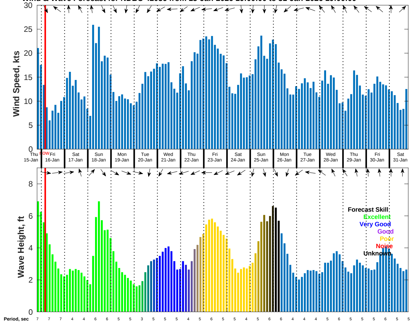
Wind & Wave Forecast for NDBC 42036 from 15-Jan-2026 19:00:00 to 31-Jan-2026 19:00:00
