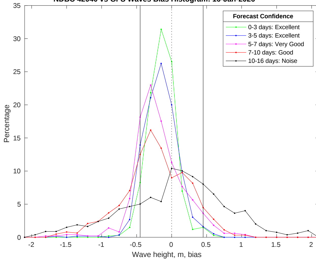
NDBC 42040 vs GFS Waves Bias Histogram: 16-Jan-2026
