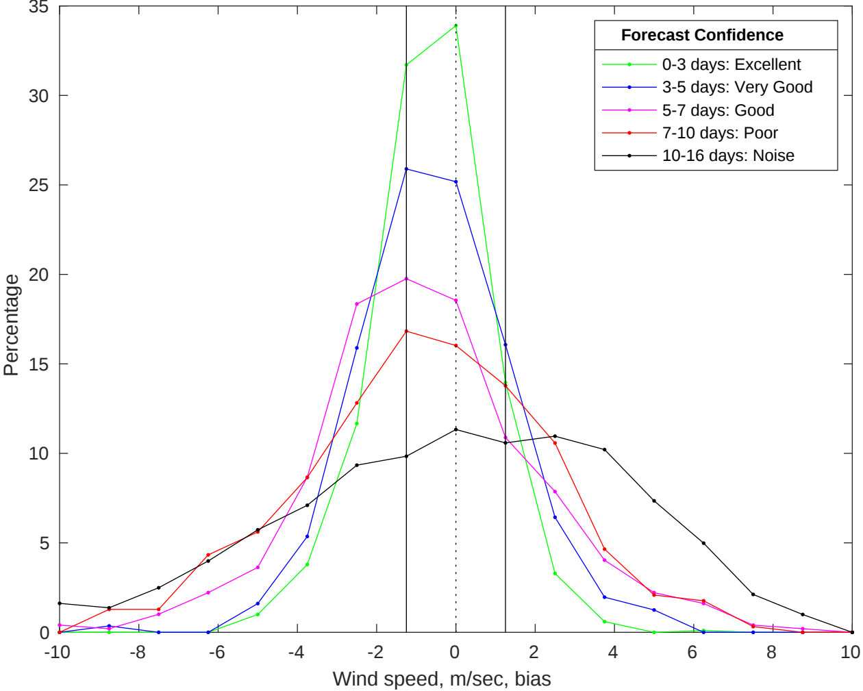
NDBC 42040 vs GFS Winds Bias Histogram: 16-Jan-2026
